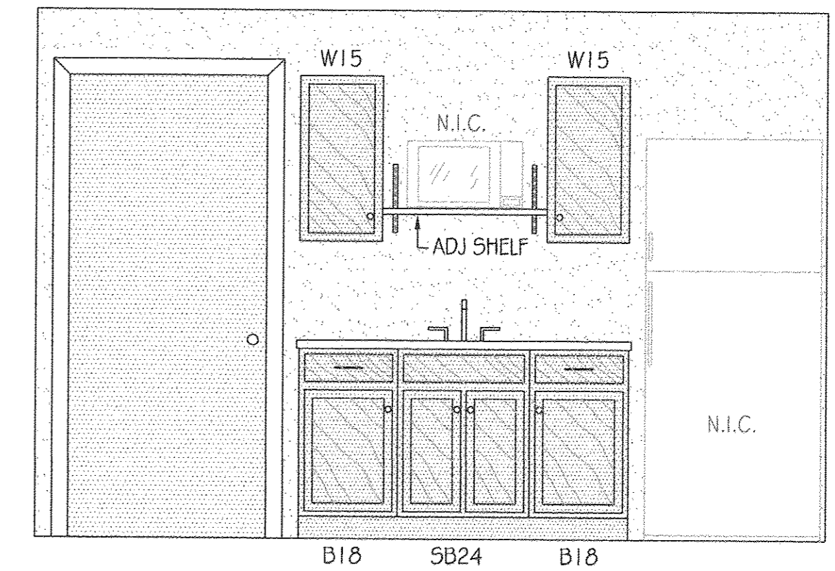
BREAK/OFFICE SCALE: 1/2" = 1'-0"
