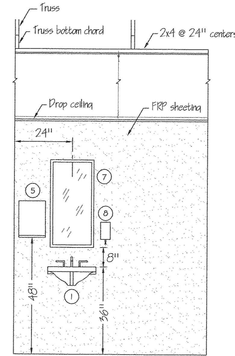
RESTROOM ELEVATIONS SCALE: 1/2" = 1'-0"
